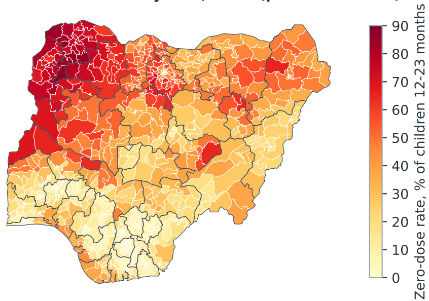
A. Zero-dose rate by LGA, 2026 (posterior mean)
