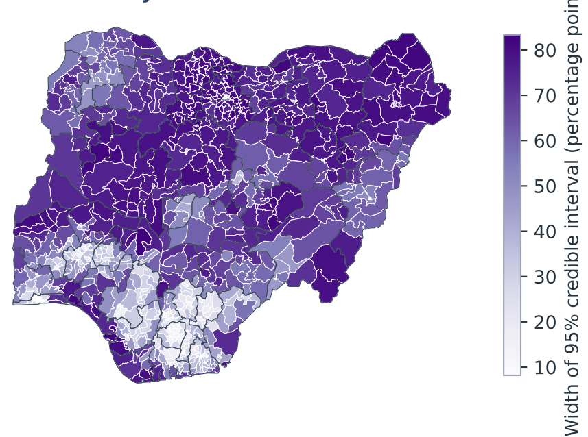
B. Uncertainty: width of the 95% credible interval
