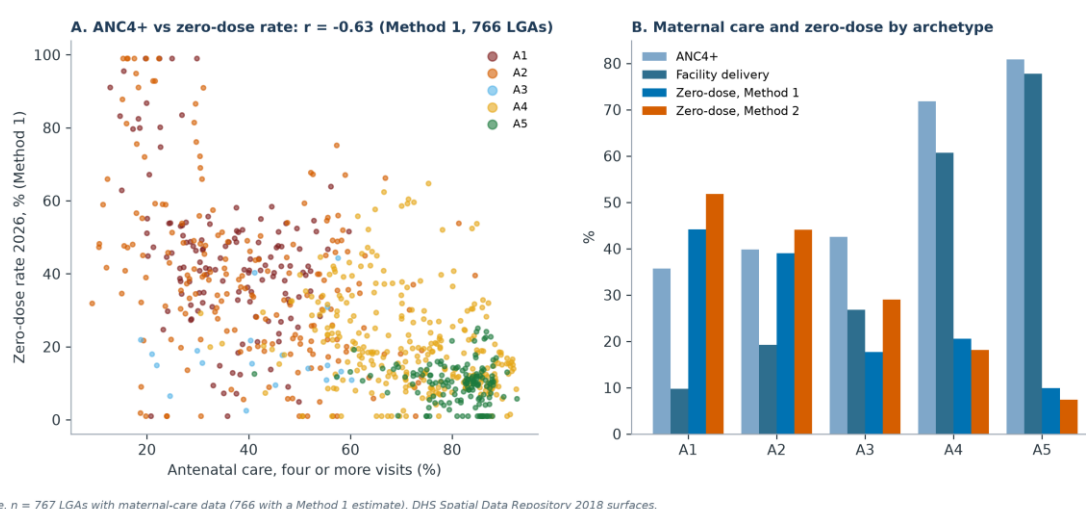
Figure 16. Antenatal care (four or more visits) against the Method 1 zero-dose rate (766 LGAs), and maternal-care indicators and zero-dose under both methods, by archetype.
