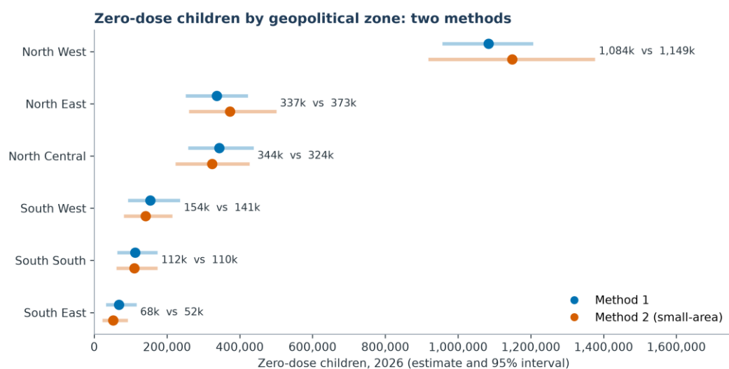
Figure 16h. Modelled zero-dose children by zone, 2026, under both methods, with 95% intervals.
