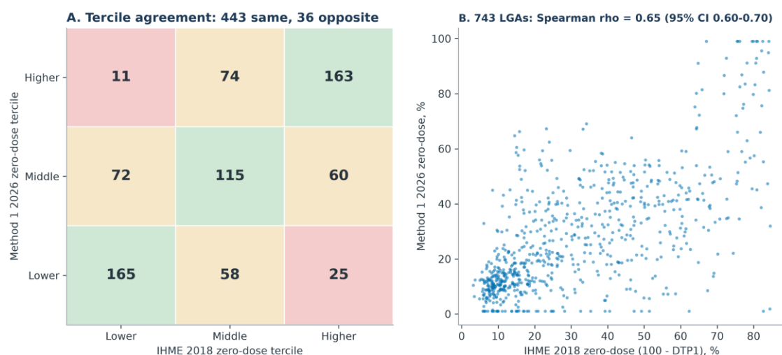
Figure 26. Convergent validity: the 2026 Method 1 LGA estimates against the IHME Local Burden of Disease DTP1 surface ( \rho = 0.65 ).
