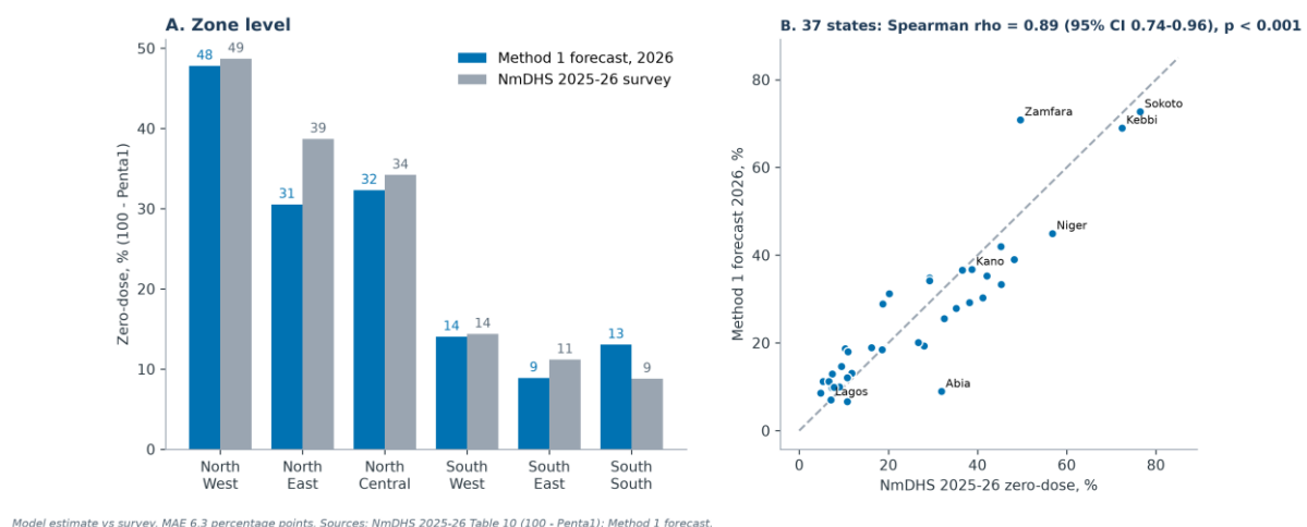
Figure 25. Prospective validation: the 2026 Method 1 state forecasts against the NmDHS 2025-26 survey, 37 states ( \rho = 0.89 ).
