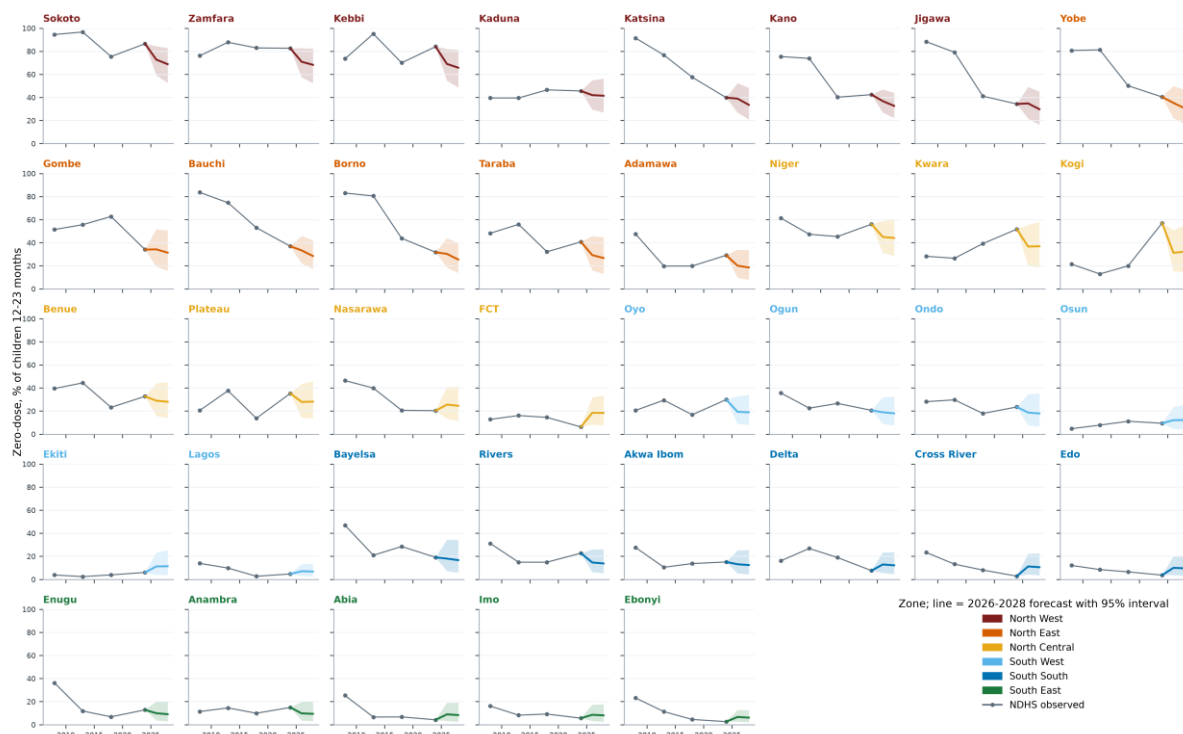
Figure 9. State-level zero-dose: NDHS 2008-2024 observations and Method 1 forecasts for 2026-2028 (shaded bands are 95% credible intervals).
