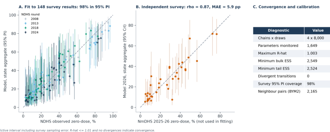
Figure 16f. Method 2 model performance: fit to all NDHS rounds, independent NmDHS 2025-26 check, and Markov chain Monte Carlo diagnostics.
