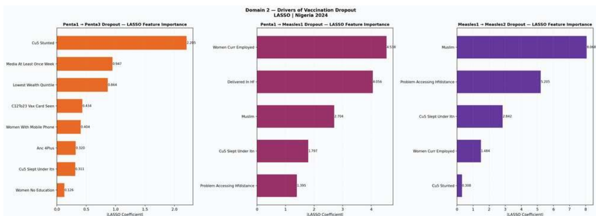
Figure 4. LASSO feature importance for the three dropout transitions.
