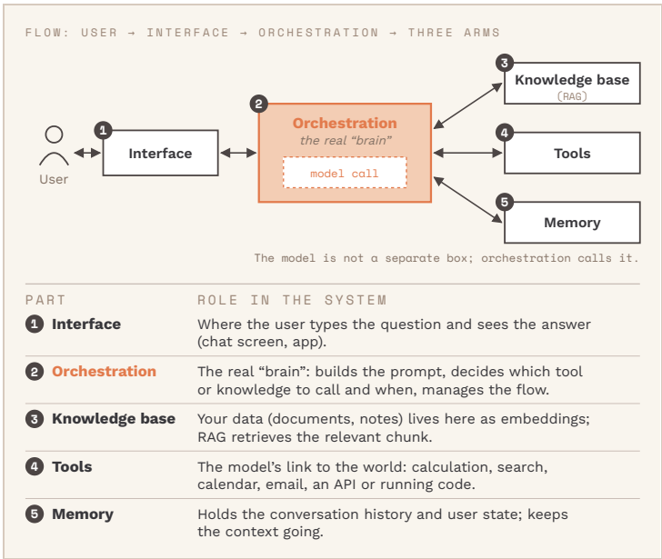
Figure 6.4 · The parts of an AI application
