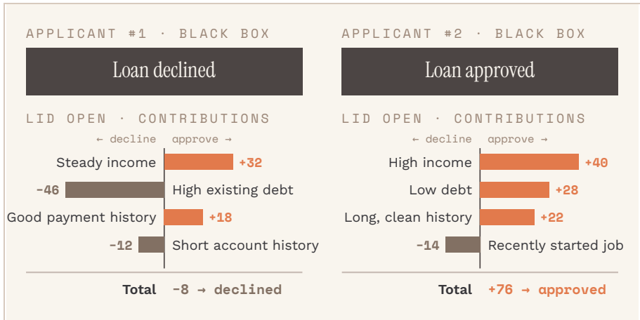
Figure 7.2 · White box: explain the decision
