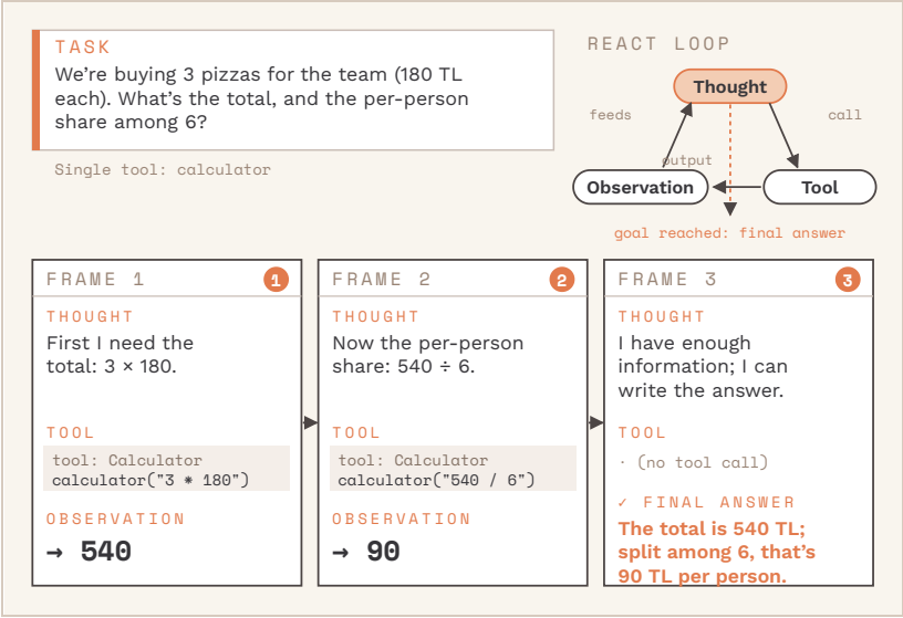
Figure 6.3 • Watch an agent
