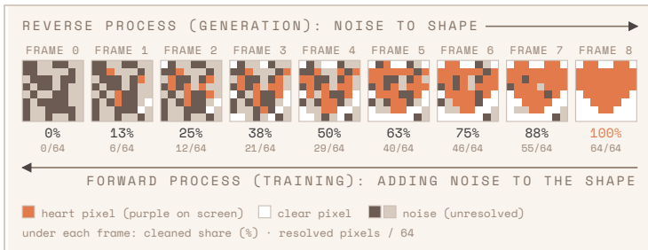
Figure 5.6 · From noise to image
