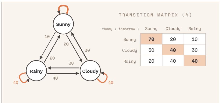
Figure 2.4 · A weather Markov chain
