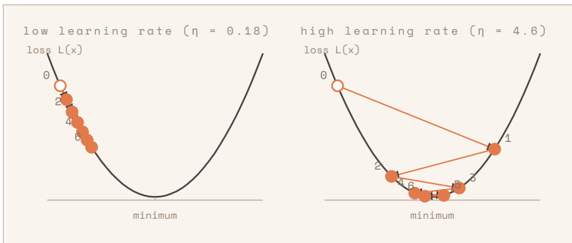
Figure 3.5 · Descending the loss valley
