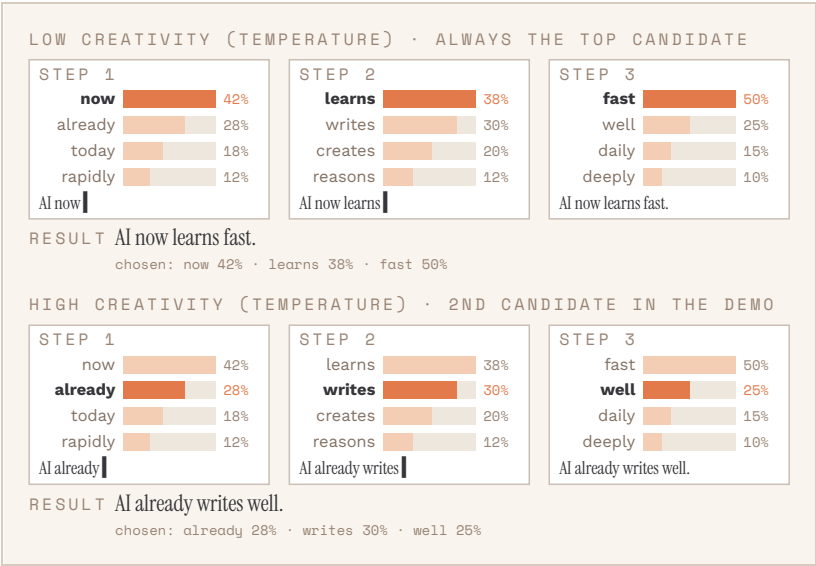
Figure 5.4 • Generate word by word
