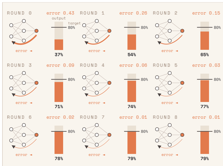
Figure 4.3 • Learn from error (animation)
