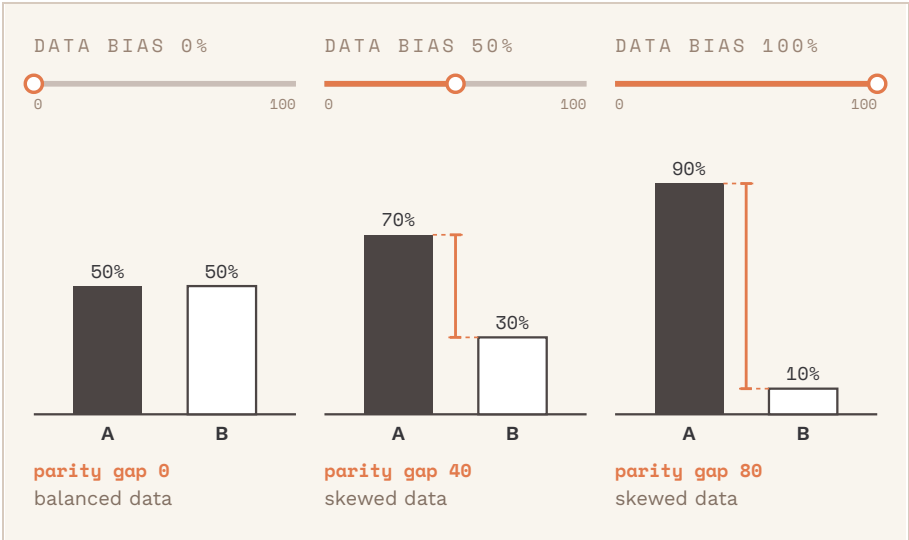
Figure 7.1 · A bias simulation
