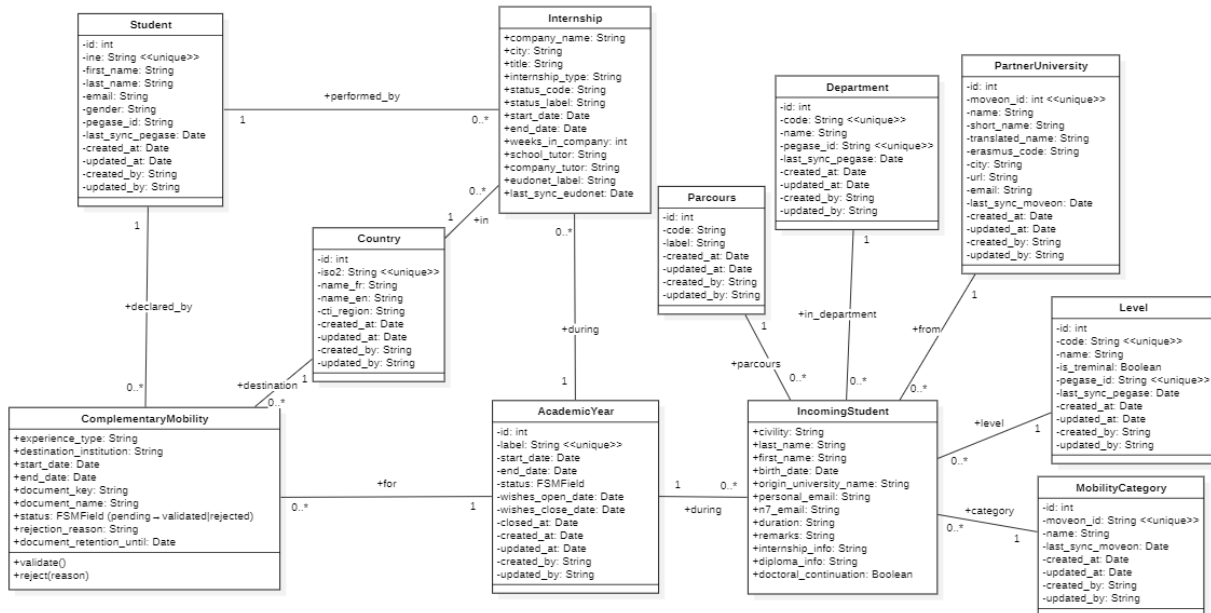
FIGURE 5.14 – Diagramme de classes : Sprint 4
