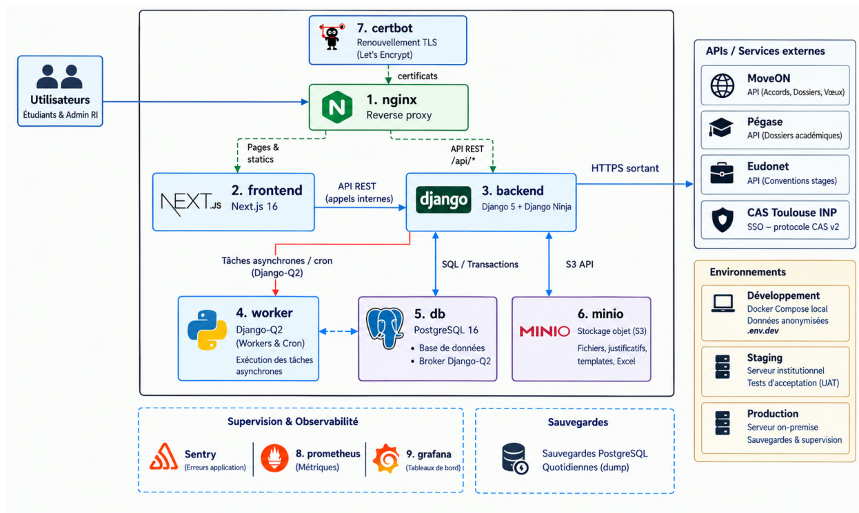
FIGURE 3.3 – Architecture physique
