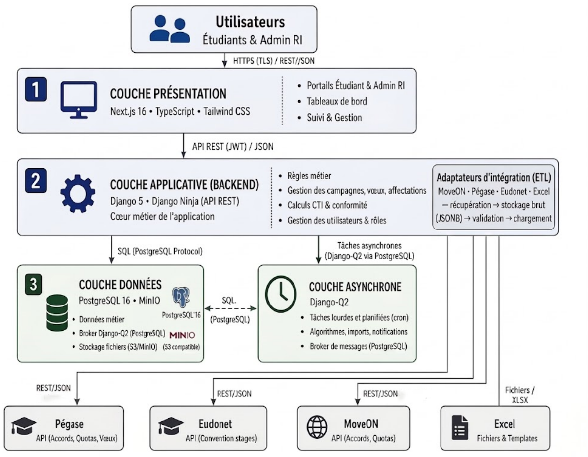
FIGURE 3.1 – Architecture logicielle
