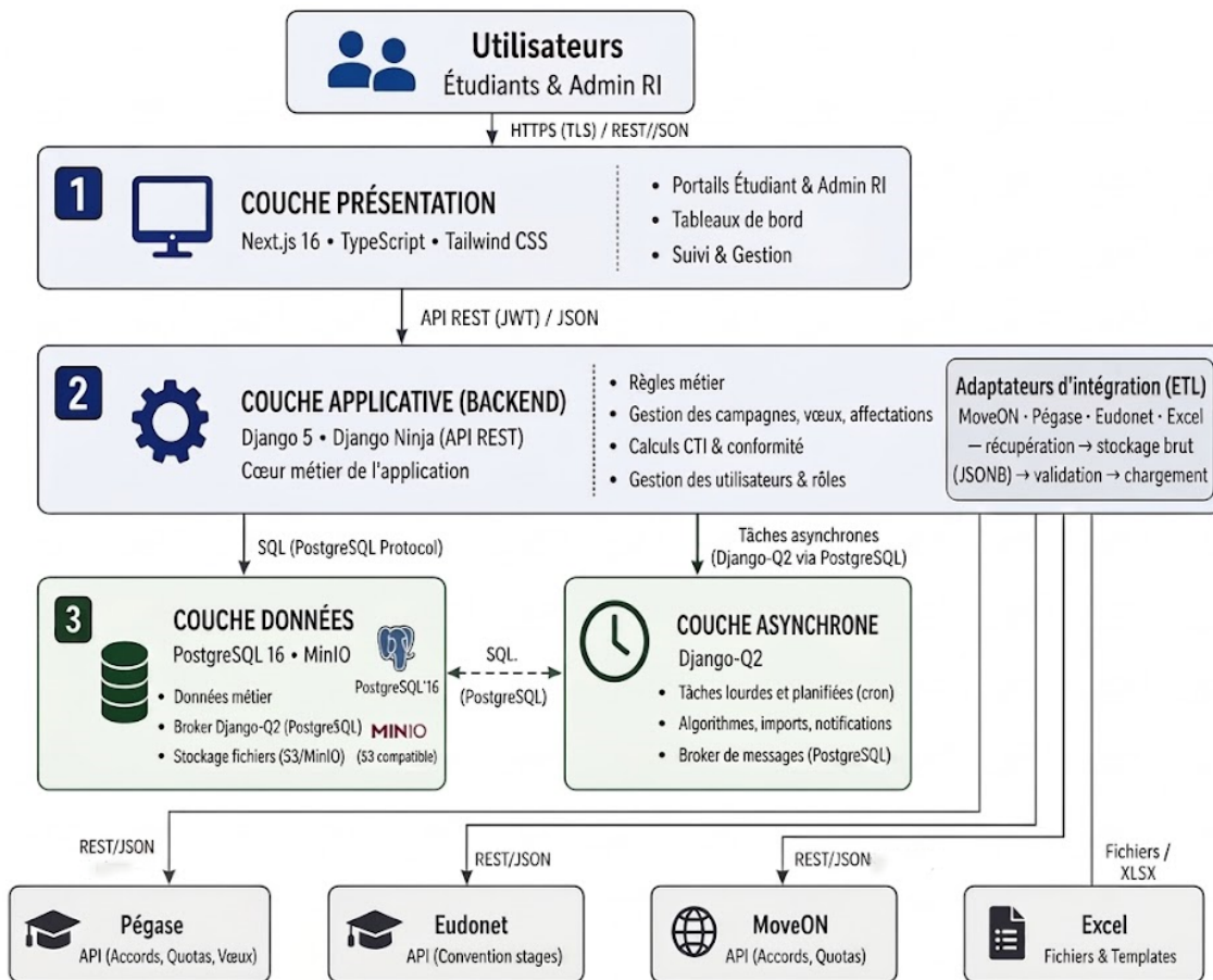
FIGURE 3.1 – Architecture logicielle
