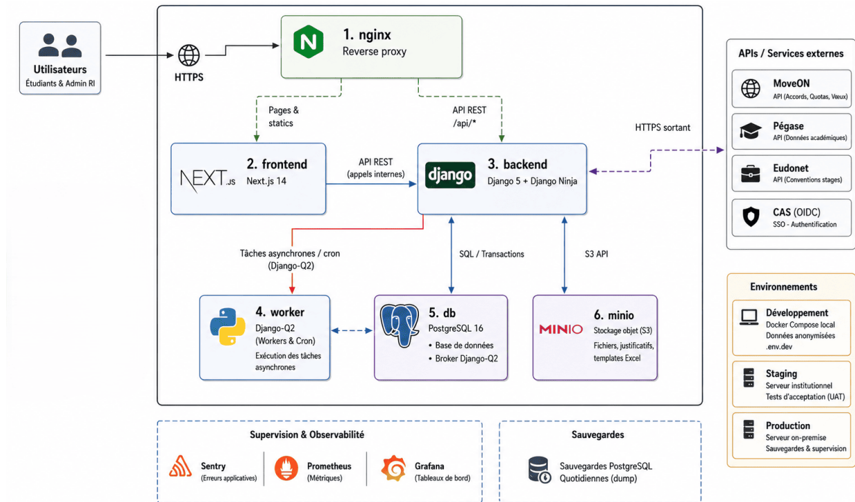
FIGURE 3.2 – Architecture physique
