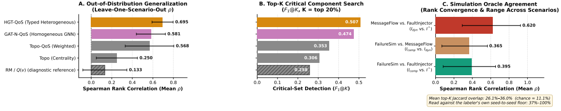
Figure 3: Results at a glance, Application population. (A) Out-of-distribution rank correlation per predictor across the twelve LOSO folds. (B) Critical-set identification at K = 20\% . (C) Pairwise rank agreement between the three simulation oracles, against the chance baseline. Panels A and B are read directly from the same artifact as Table 8 and panel C from that behind Table 10; the ordering shown is whatever the data gives, which is why the untrained Topo-QoS baseline sits third rather than last.
