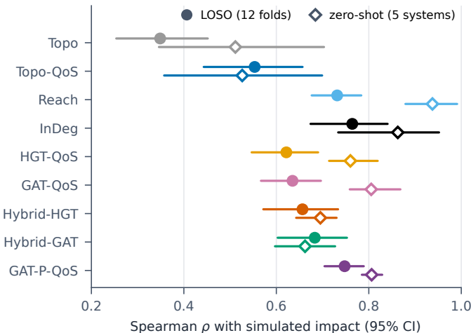
A. Dependency counts and dependency-graph learners lead
