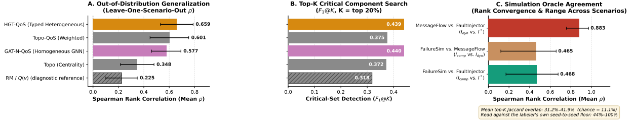
Figure 3: Results at a glance, evaluated on the Application population. (A) Out-of-distribution rank correlation per variant across twelve LOSO folds (whiskers denote \sigma ). (B) Critical-set identification at K = 20\% . (C) Pairwise agreement across the three simulation oracles.
