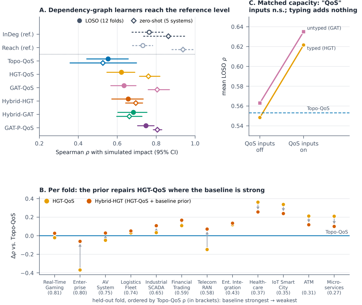
Figure 4: Main results at a glance, Application population. (A) Mean Spearman \rho with 95% bootstrap intervals under LOSO (filled circles; Table 5) and zero-shot on five system models (open diamonds). Grey hollow markers are reference rankings that restate I^* 's propagation rule ( InDeg , Reach ), not predictors; the neural model reading the dependency graph ( GAT-P-QoS ) comes close to InDeg ; the two are statistically indistinguishable but not equivalent. (B) Per held-out fold, the gain of HGT-QoS and of Hybrid-HGT over Topo-QoS . (C) Cell means of the capacity- and channel-matched 2 \times 2 (Table 7): the "QoS" inputs, which include a QoS-weighted in-degree column, raise both models by about 0.07 (not significant after Holm), while typed and untyped configurations are indistinguishable; with w_{in} held in both arms the "QoS" effect falls to +0.030 (Table 8).
