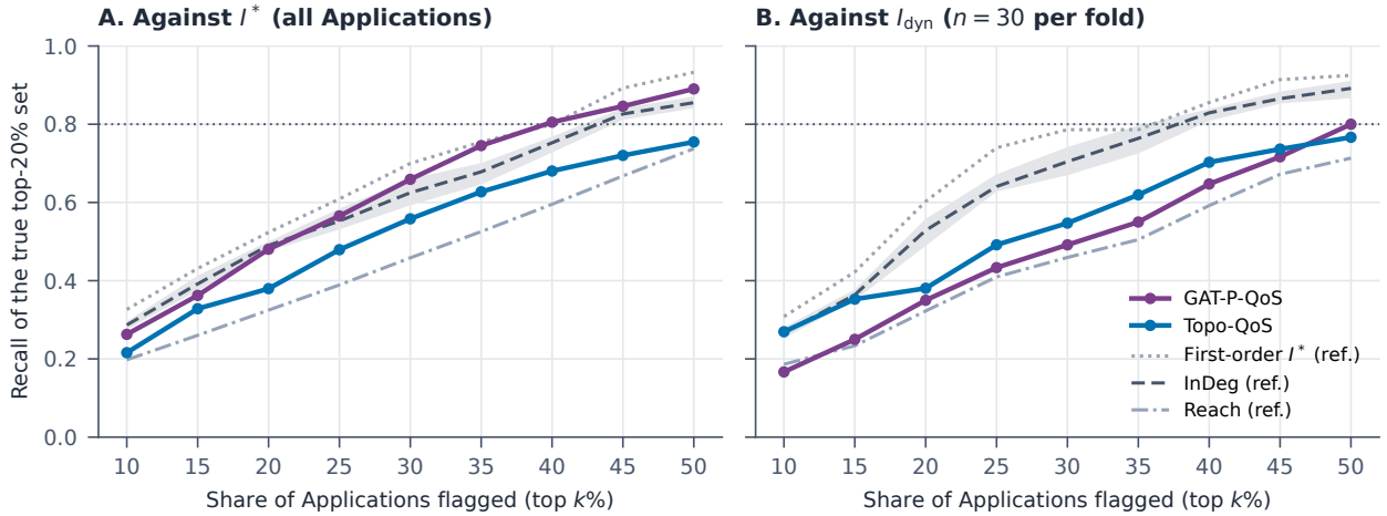
Figure 5: Recall of the true top-20% set (tie-inclusive) by each ranker’s top k\% , mean over the twelve LOSO folds, against I^* (left) and the exploratory developmental sample ( I_{\text{dyn}} on n = 30 Applications per fold; right). The right panel was drawn before exhaustive I_{\text{dyn}} labels existed and has not been redrawn; Table 6 reports the exhaustive N = 1,321 population. Ties are resolved in expectation over random tie-breaking; grey dashed curves are reference rankings that restate I^* ’s rule, and the shaded band gives InDeg ’s optimistic and pessimistic bounds. Reach , whose scores tie heavily, has much wider bounds (0.12–0.80 at k = 20\% on I^* ), so its expected curve is the only meaningful summary. The dotted line marks 80% recall.
