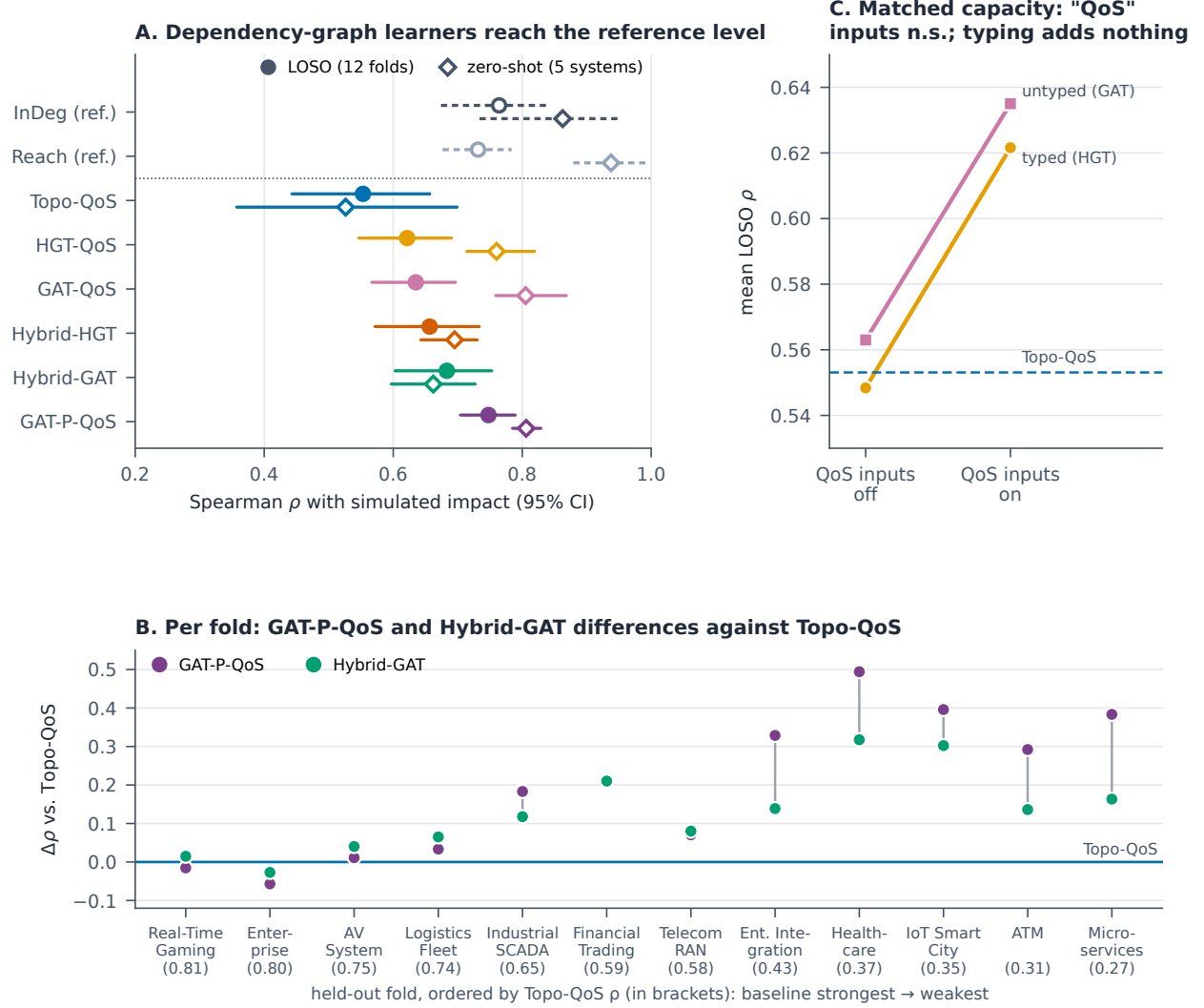
Figure 4: Main results for the Application population. (A) Mean Spearman \rho with 95% bootstrap intervals under LOS0 (filled circles; Table 5) and zero-shot on five system models (open diamonds); grey hollow markers are references that restate I^* 's rule (InDeg, Reach). GAT-P-QoS is not distinguishable from InDeg, and equivalence within \pm 0.05 is not established (TOST p = 0.17 ). (B) Per-fold improvement of GAT-P-QoS and Hybrid-GAT over Topo-QoS. (C) Cell means of the capacity-matched 2 \times 2 on the raw multigraph (Supplementary Table S25): the "QoS" inputs, which include a QoS-weighted in-degree column, raise both models by about 0.07 (not significant after Holm), falling to +0.030 with w_{\text{in}} held in both arms (Table 7).
