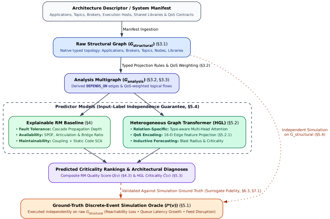
Figure 1: End-to-end architecture of the Software-as-a-Graph (SaG) framework: architecture manifest ingestion → typed multigraph → logical dependency projection → dual predictor paths (explainable RM baseline and Heterogeneous Graph Transformer) validated against independent discrete-event simulation.
