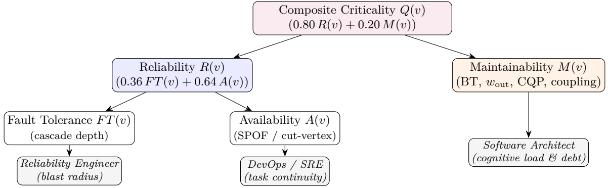
Figure 2: The hierarchical RM Diagnostic Attribution Model and stakeholder role mapping. Each arrow is a scoring dependency computed by the same deterministic pass, not a post-hoc explanation of a separately trained model.
