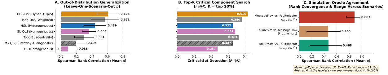
Figure 3: Results at a glance, all on the Application population. (A) Out-of-distribution rank correlation per variant, whiskers showing \sigma across the eight LOSO folds; note that the training-free Topo-QoS baseline places second. The hatched bar is RM/Q(v), the Pathway A diagnostic reference of Section 1.2 — shown for context, not as a competing ranking predictor. (B) Critical-set detection at K = 20\% , same hatching convention. (C) Agreement between the three simulation oracles, whiskers showing the observed range across scenarios; the annotation gives top- K set agreement against both chance and the labeler’s own seed-to-seed floor.
