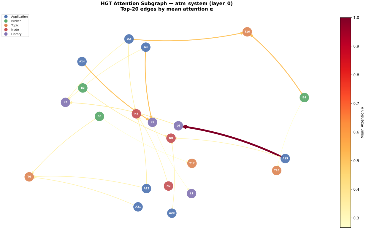
Figure 5: Relational attention extracted from the trained HGT on the ATM case study. The highest-weighted channels are USES (Application → shared Library) and ROUTES (Broker → Topic) rather than direct publish/subscribe edges, matching the shared-library blast-radius and broker-centrality pathways found by the edge-removal analysis.
