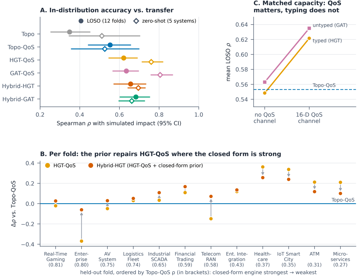
Figure 5: Main results at a glance, Application population. (A) Mean Spearman \rho with 95% bootstrap intervals under LOS0 (filled circles; CPU sweeps of Table 8) and zero-shot on the five system models (open diamonds). The hybrids lead on unseen synthetic architectures; the pure learned engines transfer best. (B) Per held-out fold, the gain of HGT-QoS and of Hybrid-HGT over Topo-QoS; the arrow shows what the closed-form prior changes. It removes the learned engine’s losses where the closed-form engine is strongest (Enterprise, Telecom RAN) and trims its largest gains where it is weakest. (C) Cell means of the capacity- and channel-matched 2 \times 2 (Table 9): the QoS channel raises both models by about 0.07, while the typed and untyped lines stay together.
