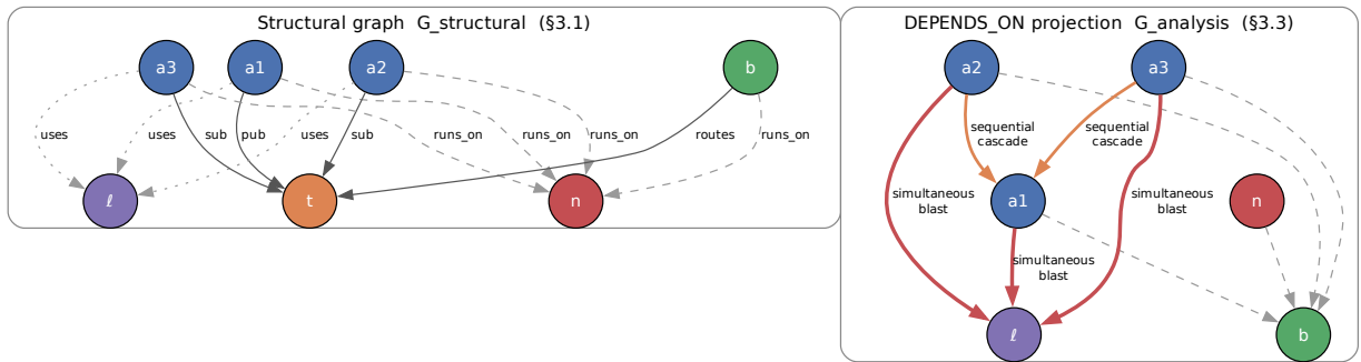
Figure S3: Running example: the raw structural graph (left) and the DEPENDS_ON projection derived from it (right). The projection makes implicit runtime dependencies explicit—a subscriber depends on the publishers of its topics even though no structural edge joins them—while the simulators continue to operate on the structural view alone.
