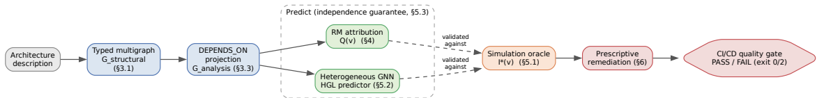
Figure 1: End-to-end architecture of the Software-as-a-Graph (SaG) framework: architecture manifest ingestion → typed multigraph → logical dependency projection → dual predictor paths (interpretable RM baseline and Heterogeneous Graph Transformer) validated against independent discrete-event simulation.
