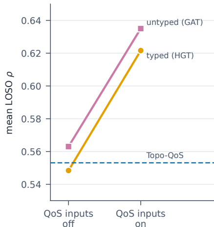
C. Matched capacity: "QoS" inputs n.s.; typing adds nothing
