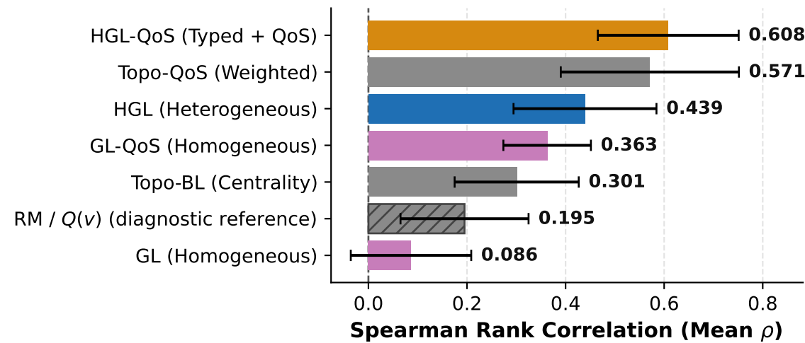
A. Out-of-Distribution Generalization (Leave-One-Scenario-Out \rho )
