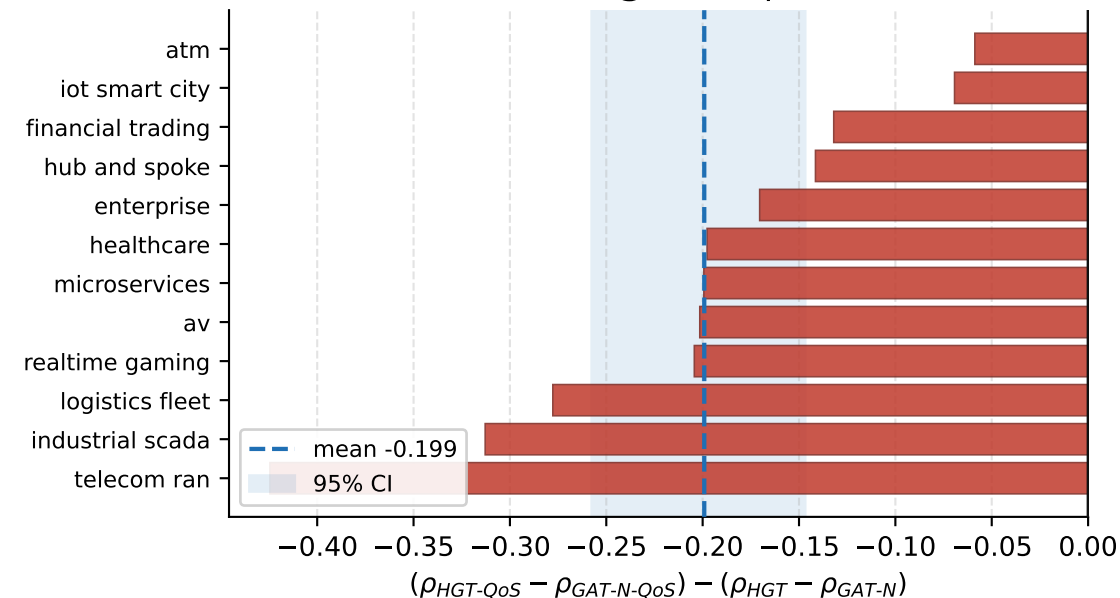
D. Typing \times QoS Interaction (12/12 folds negative, p = 0.0005 )
