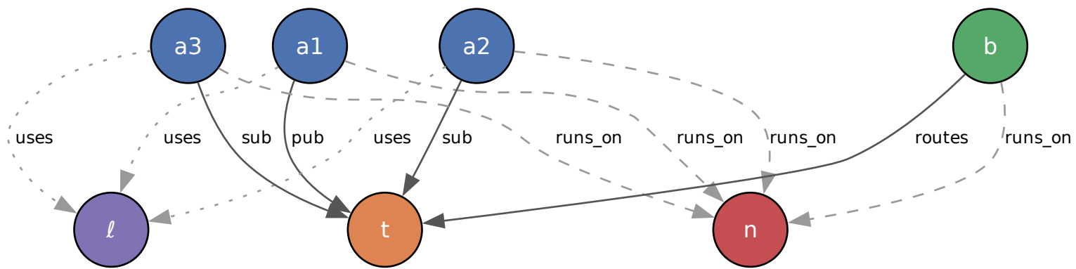
Structural graph G_{\text{structural}} (§3.1)
