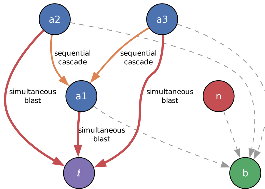
DEPENDS_ON projection G_{\text{analysis}} (§3.3)
