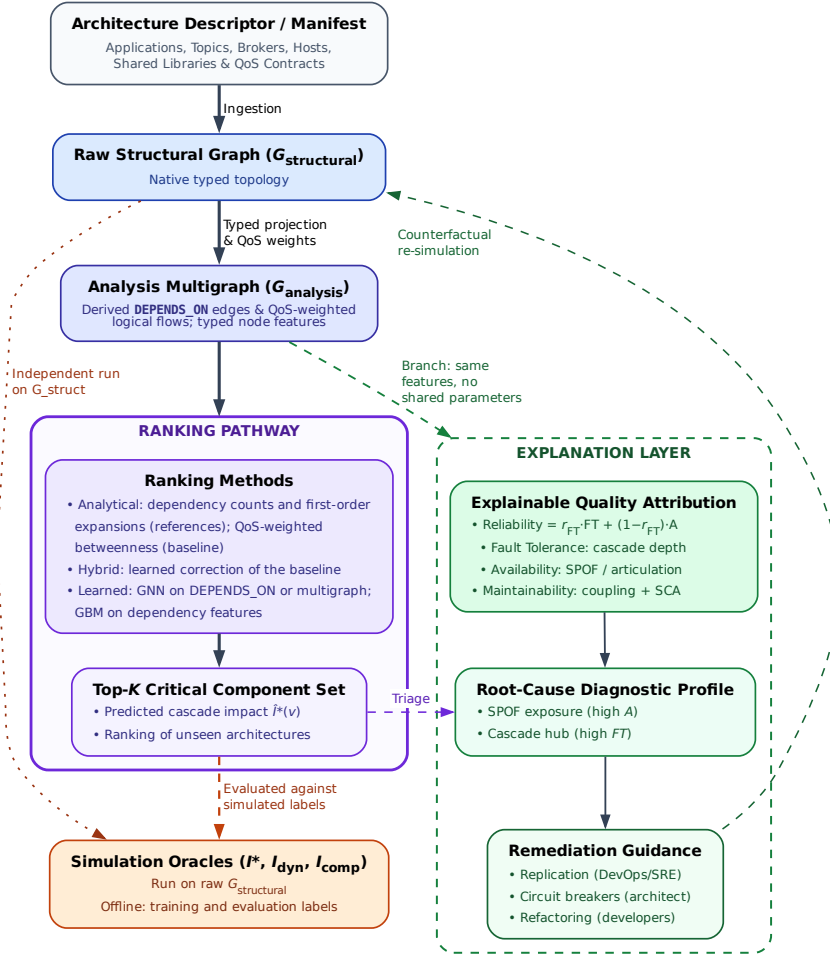
Figure 1: End-to-end architecture of the SaG framework. The ranking pathway runs down the center: manifest ingestion, typed structural multigraph ( G_{\text{structural}} ), DEPENDS_ON logical dependency projection ( G_{\text{analysis}} ) with typed node properties, the ranking methods (analytical, hybrid, and learned; Figure 3), and the ranked critical set. The same dependency graph supports all three ranking methods. The dashed edge marks the simulation oracles, which operate strictly on G_{\text{structural}} , provide training and evaluation labels offline, and do not participate in inference. The proposed explanation layer (not evaluated) reads G_{\text{analysis}} , shares no parameters with the rankers, and applies to components after they have been ranked; no ranker output flows into it.
