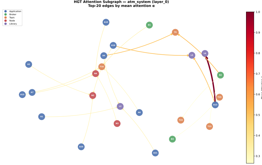
Figure S2: Relational attention on the ATM case study, from a three-layer HGT trained for 100 epochs on this scenario alone (seed 42) — not the predictor evaluated in Sections 7.1–7.3 of the main manuscript. Mean \alpha spans 0.113–0.222 across the eight relation types and is governed substantially by destination in-degree. A qualitative illustration on one topology, not evidence of general relation prioritization.
