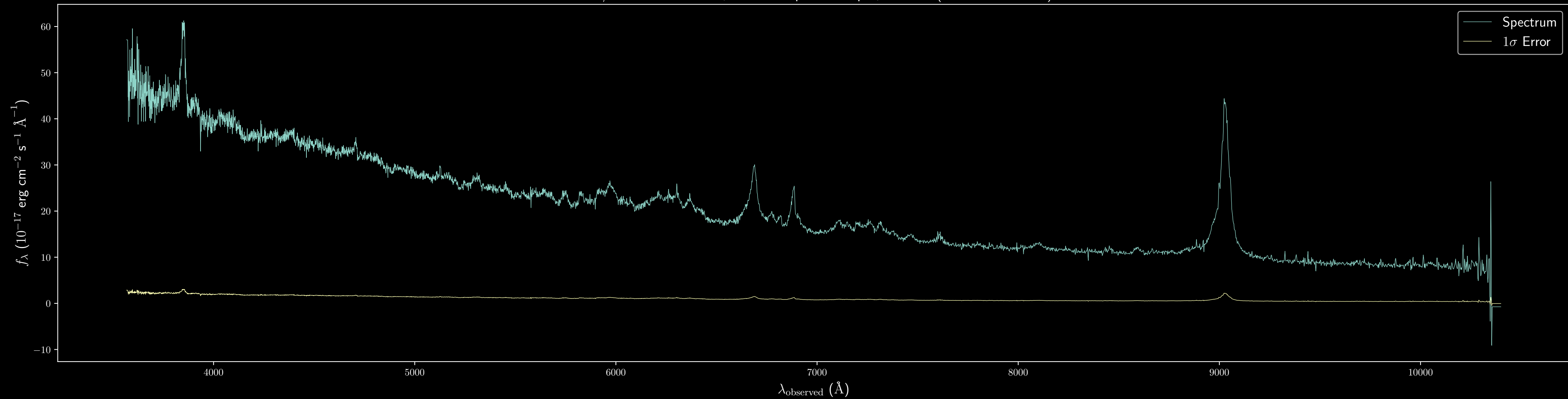
Keck/LRIS Un-normalized, Observed Spectrum Input, z=0.377 (Sexton et al. 2019)
