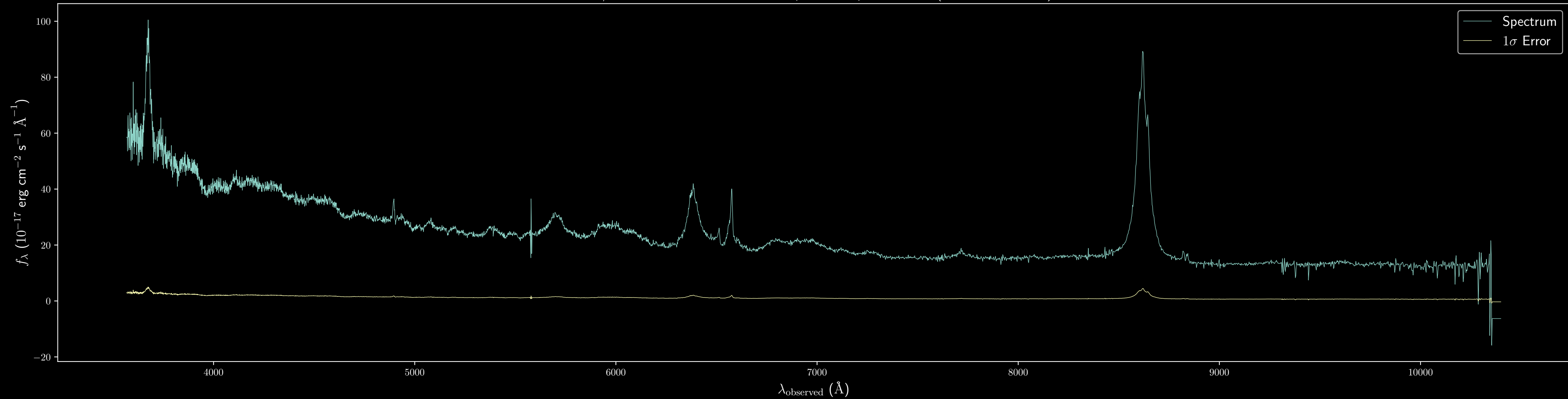
Keck/LRIS Un-normalized, Observed Spectrum Input, z=0.314 (Sexton et al. 2019)
