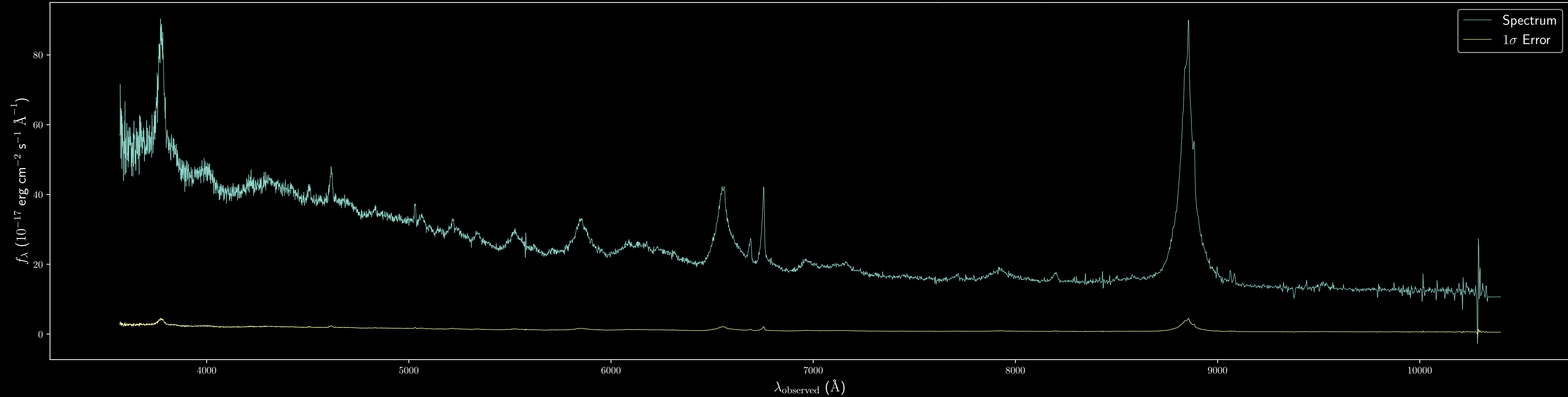
Keck/LRIS Un-normalized, Observed Spectrum Input, z=0.349 (Sexton et al. 2019)
