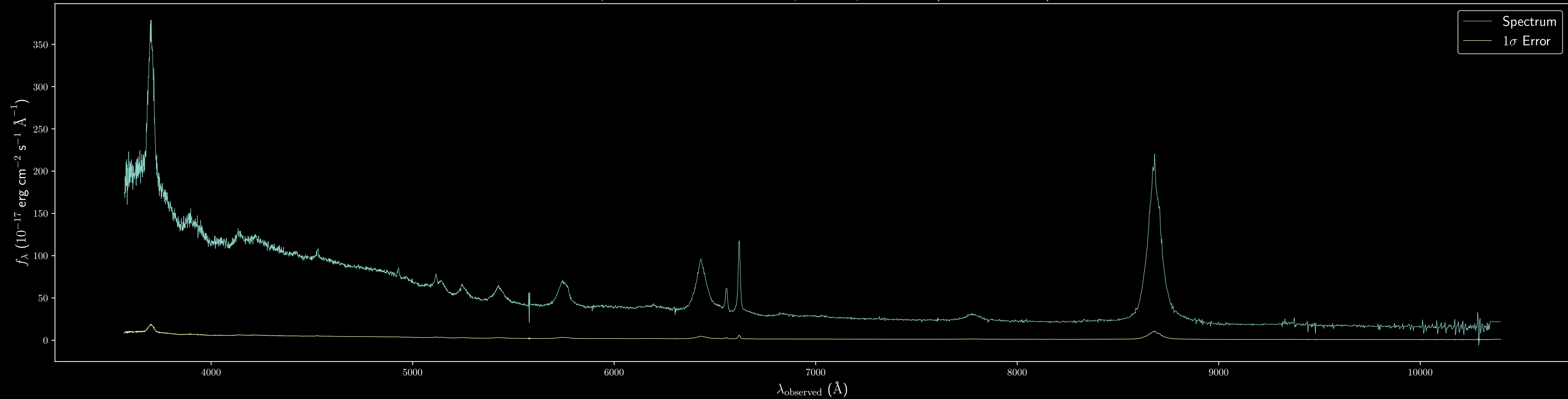
Keck/LRIS Un-normalized, Observed Spectrum Input, z=0.323 (Sexton et al. 2019)
