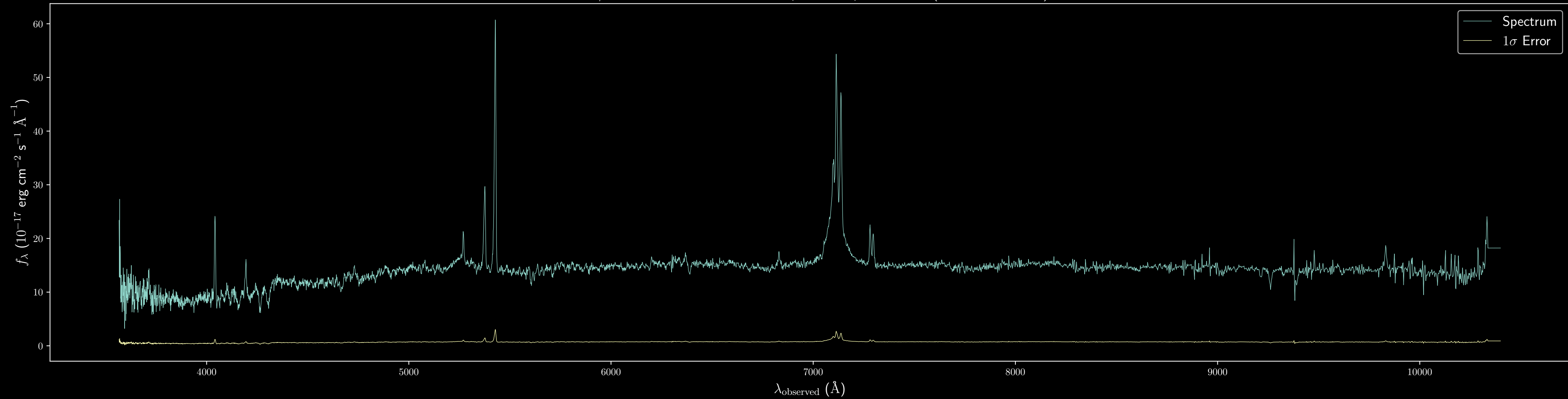
Keck/LRIS Un-normalized, Observed Spectrum Input, z=0.083 (Sexton et al. 2019)
