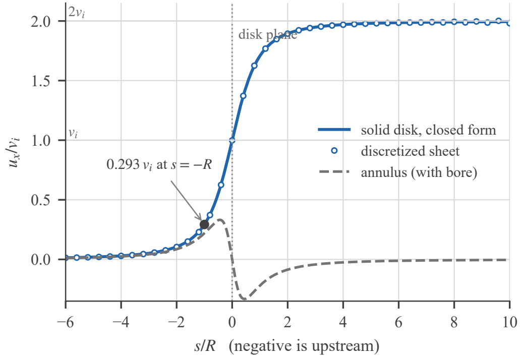
Figure 2. Axial induction on the disk axis. The discretized sheet (circles) against the closed form of Eq. (3) (solid), with the annulus (dashed) showing the reversal inside the bore that Eq. (7) predicts. Negative s is upstream — the half of the field a wake-only model does not carry, and the half this paper depends on.
