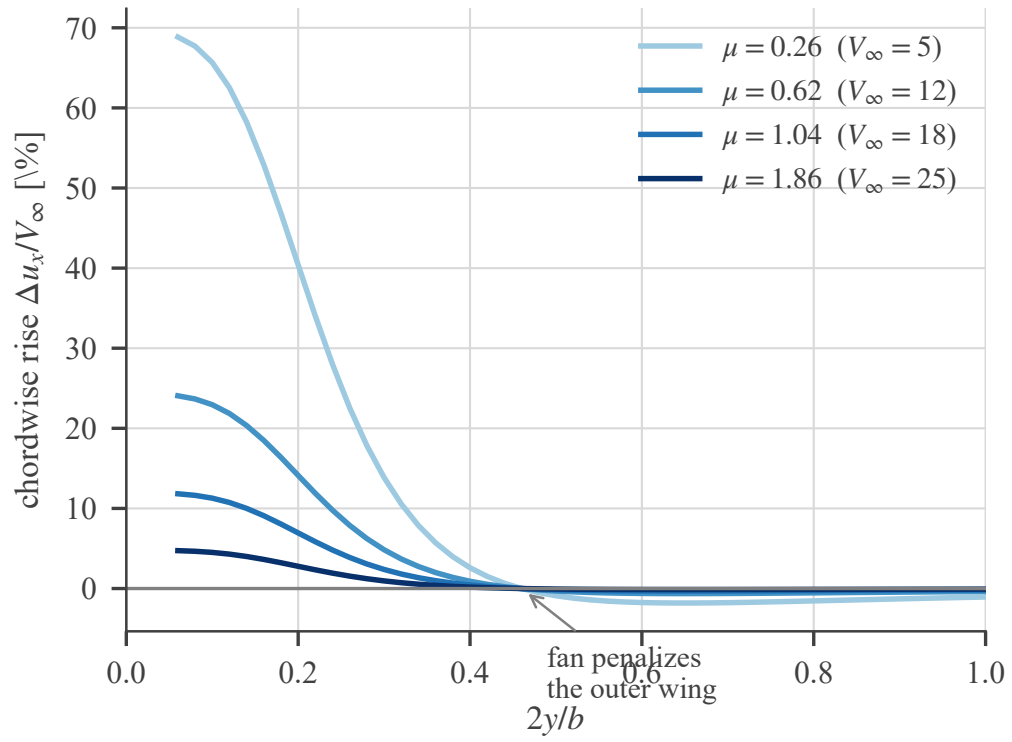
Figure 3. The chordwise rise across the span. The benefit is concentrated inboard — over the stations that separate first — and reverses beyond 2y/b \approx 0.4 , where the wing lies outside the fan’s streamtube and meets its return flow.
