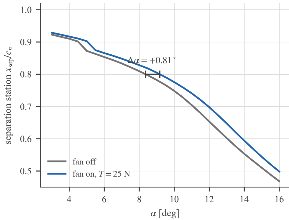
Figure 4. Separation station against incidence, fan off and on, at V_\infty = 12 m/s. The deliverable is the horizontal distance between the curves, marked at one criterion level; measuring instead where either curve crosses a fixed threshold, on a two-degree grid, returns no effect at all.
