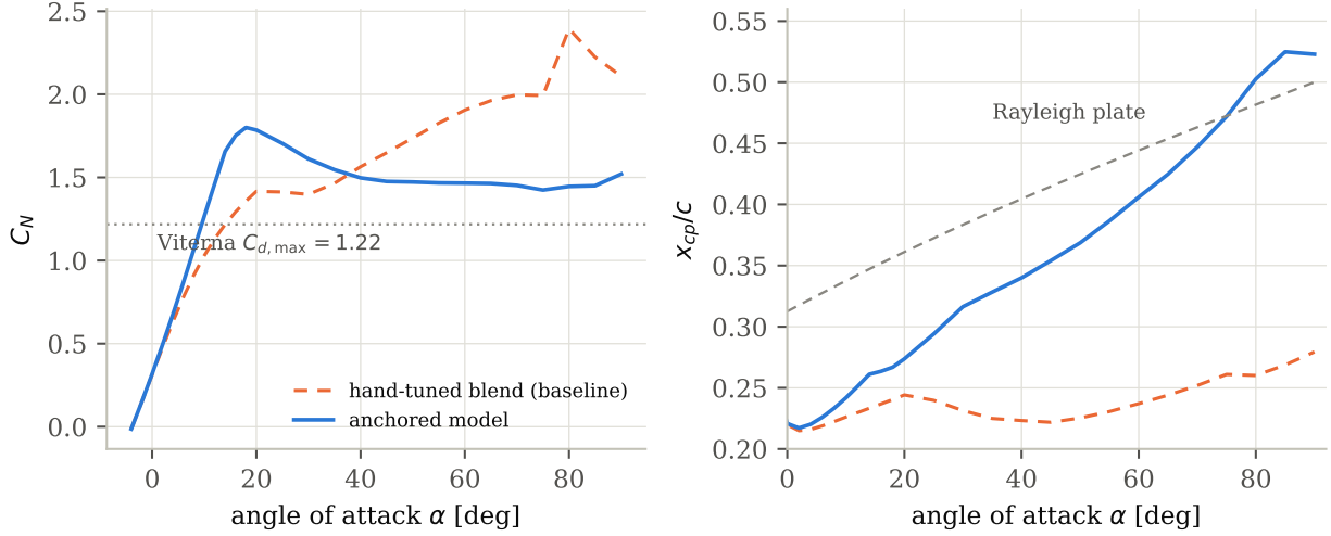
Figure 2. The \beta = 0 column against the inviscid baseline (the hand-tuned deep-stall blend this construction replaces). Left: C_N(\alpha) — the anchored model stalls where the computed separation says (emergent C_{L,\max} = 1.76 at 18^\circ ) and lands 25% above the Viterna ceiling at 90^\circ where the baseline sat 73% above. Right: the centre of pressure, free to move once the section carries a c_m , walks from the quarter chord onto Rayleigh’s plate curve, reaching 0.52c at 90^\circ .
