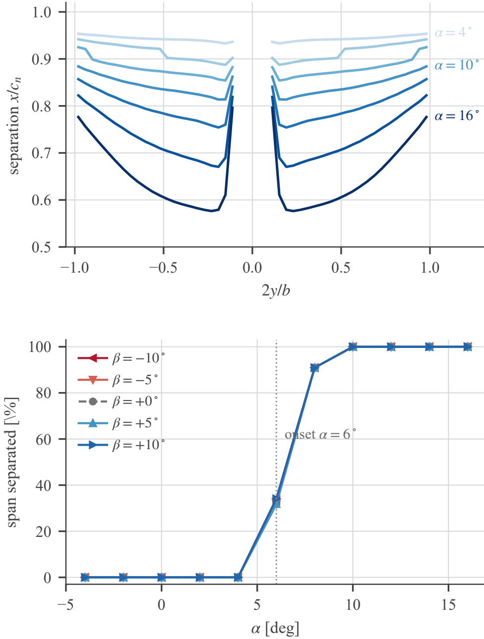
Figure 4. Upper-surface separation from the march of Section E. Top: separation station across the span at \beta = 0 , shaded light to dark with increasing \alpha ; separation is most advanced just outboard of the wing root and recovers toward the tips. Bottom: fraction of the span separated forward of x/c_n = 0.90 . The five \beta curves are all plotted and collapse — on this unswept planform the separation boundary is insensitive to sideslip, in contrast to the attachment line of Fig. 2.
