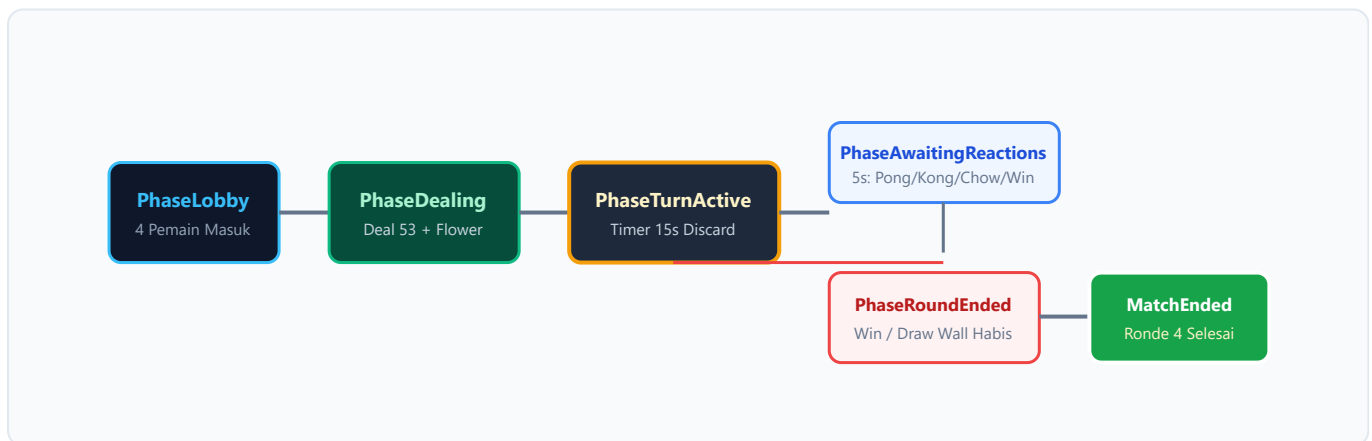
Flowchart 1: State Machine Tahapan Permainan (Game Phase)
