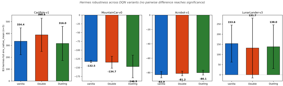
Fig. 5. B3-hermes-full mean across the three DQN variants per environment; within-environment differences are not statistically significant.
