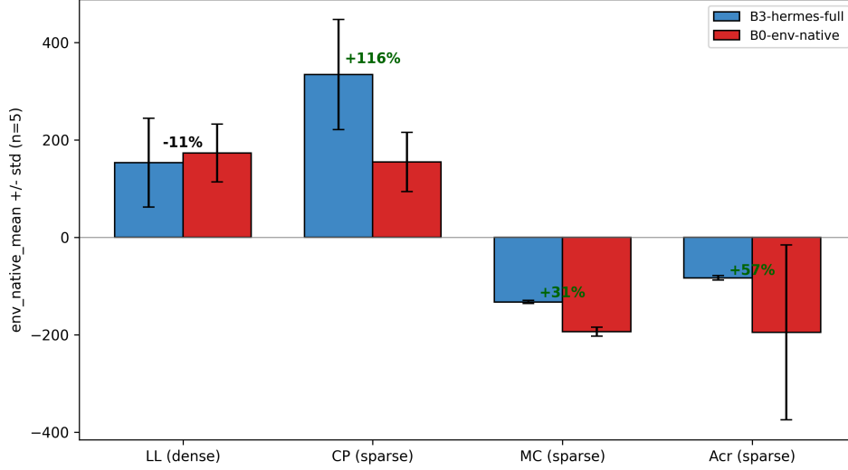
Fig. 3. Cross-environment headline comparison: B3-hermes-full versus B0-env-native across all four environments. Percentage deltas are computed on env_native_mean ; the bar pattern flips between the three sparse environments (positive \Delta ) and dense LunarLander (negative \Delta ).
