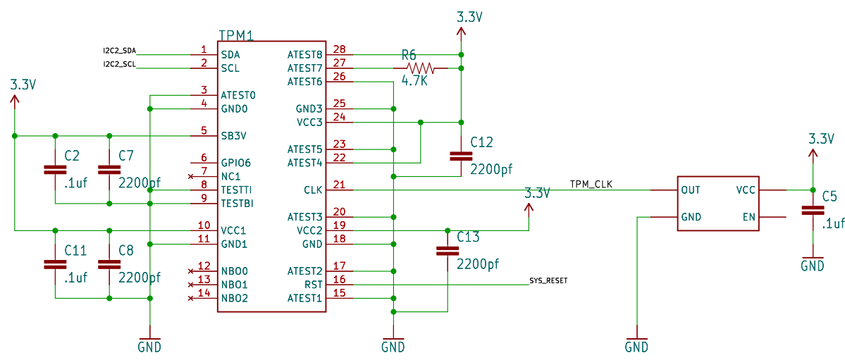
Atmel Trusted Platform Module (TPM)
