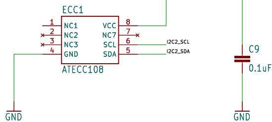
Elliptical Curve Crypto (ATECC108)
