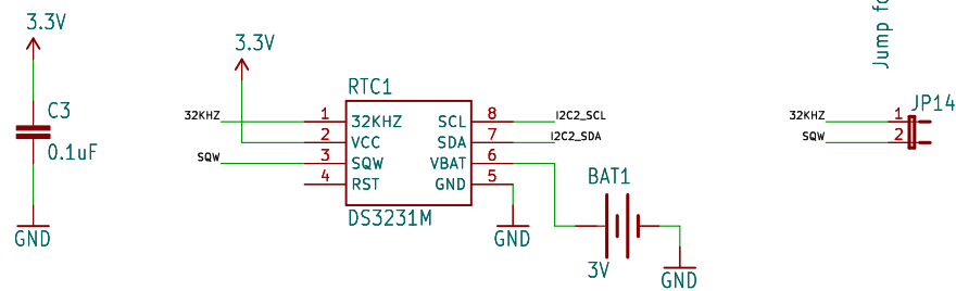
Real Time Clock (w/ Battery)
