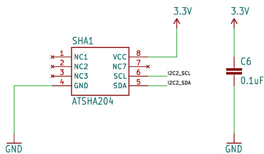
SHA-256 (ATSHA204)
