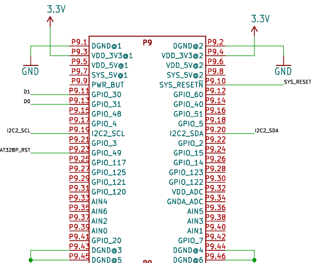
BeagleBone Black Headers
