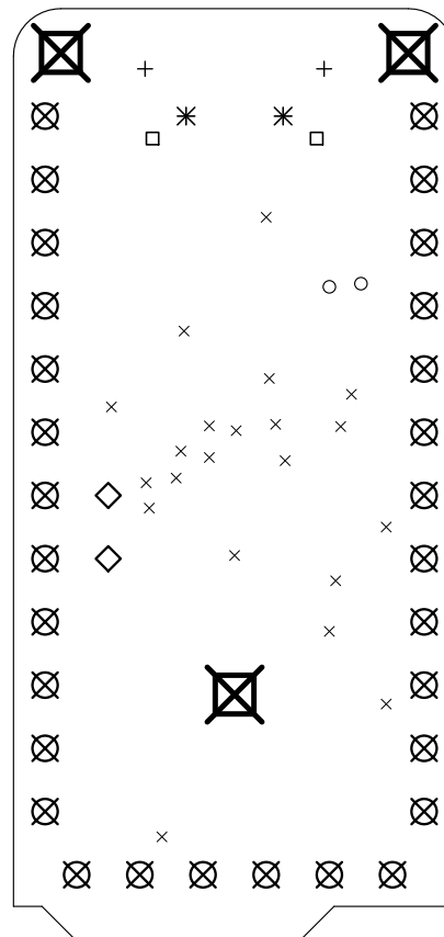
Drill Map:
