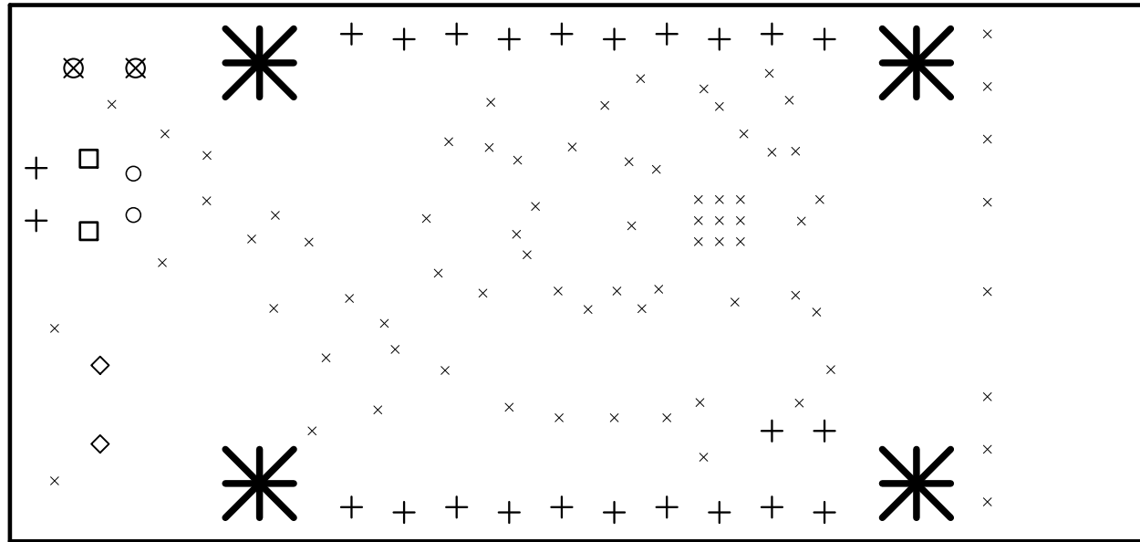
Drill Map:
