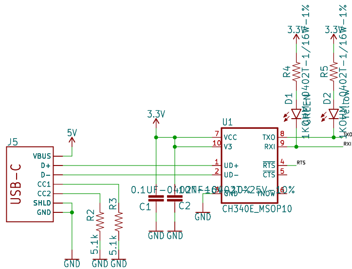
USB-to-Serial Converter
