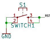
Reset Button
