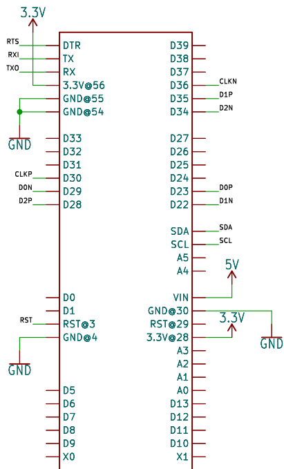
Alorium Technology Sno (Footprint)
