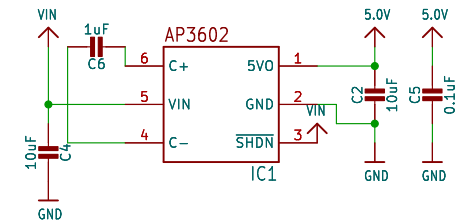
Power supply, 5V Boost Supply
