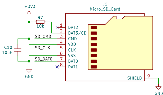
Micro-SD card
