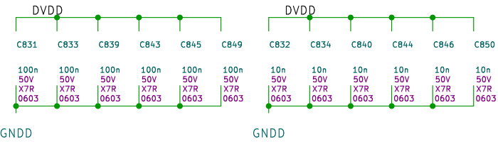
Local decoupling around U801
