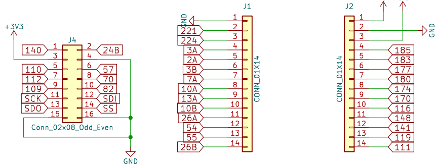
TinyFPGA Bx Pin Headers
