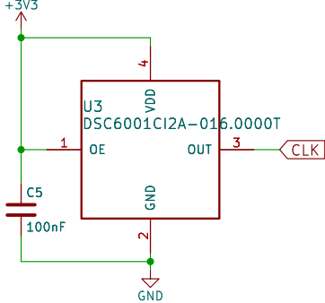
16MHz Clock
