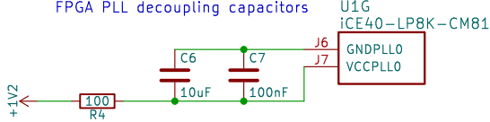
FPGA PLL decoupling capacitors
