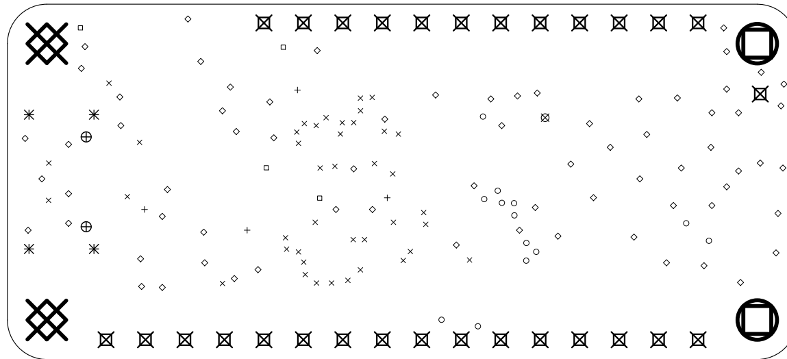
Drill Map:
