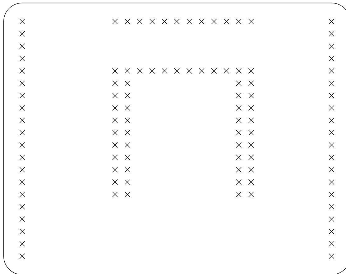
Drill Map: X 1.000mm / 0.0394" (104 holes)
