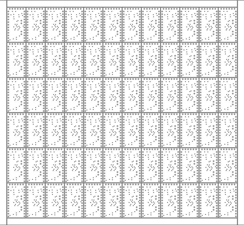
Drill Map: • 0.508mm / 0.0200" (2098 holes) ◦ 1.016mm / 0.0400" (2448 holes)
