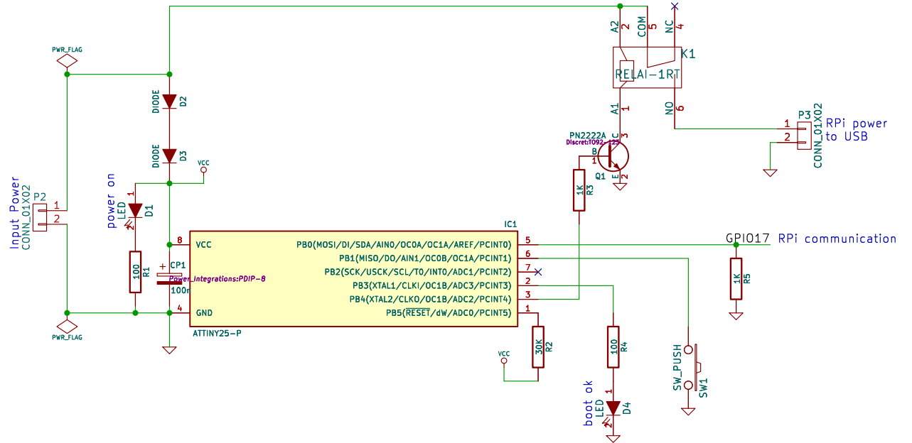
RaspBerry Pi Power Control
