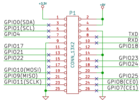
RaspBerry Pi Connector
