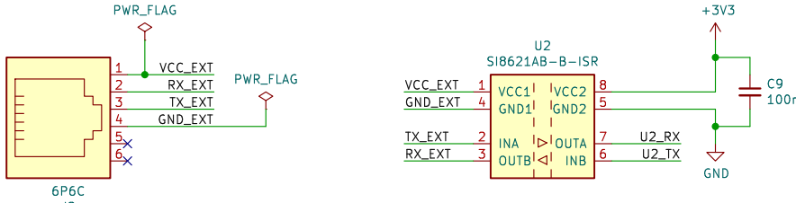
LS.one isolated UART interface
