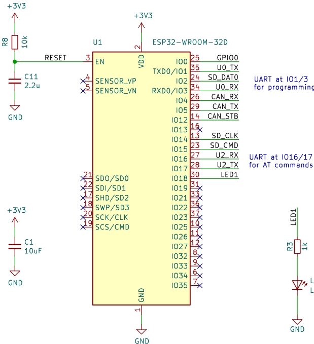
ESP32 WROOM module
