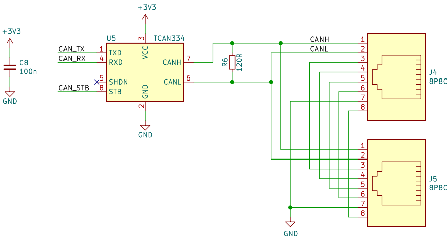
LS.bus CAN interface
