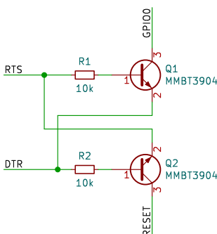
Reset and boot circuit
