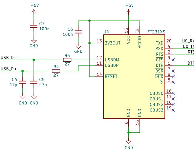
USB to UART converter for ESP programming
