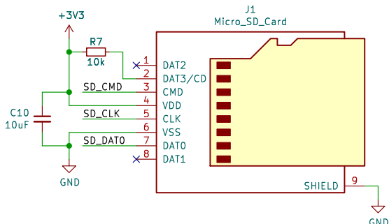
Micro-SD card
