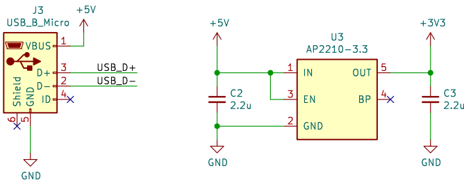
USB power supply
