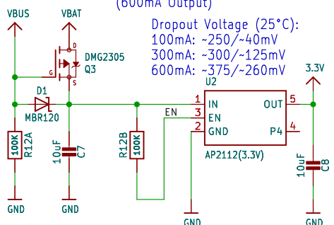
POWER AND FILTERING (600mA Output)
